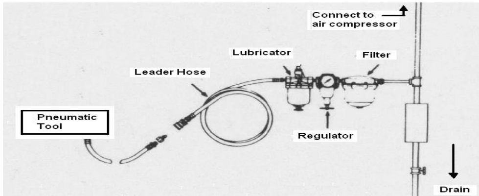
Recommended Air Line Components
